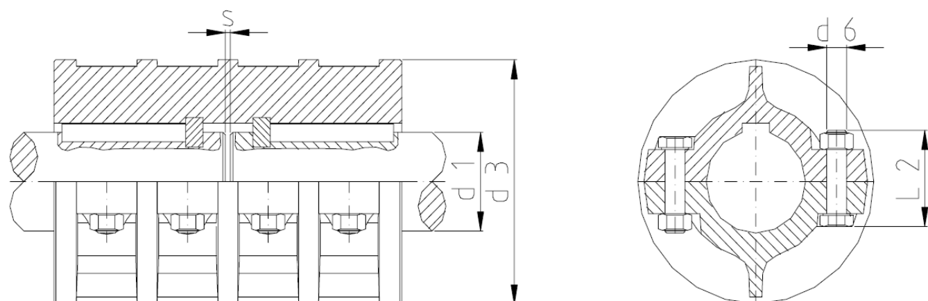
Style C for vertical design with insert rings
